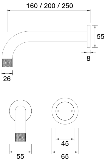
IDK Wall Mixer Basin Set 200mm outlet A38.033.1.01 - Chrome
