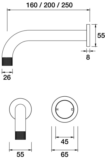
IDK Wall Mixer Basin Set 250mm outlet A38.033.3.01 - Chrome
