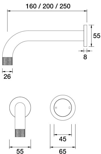
IDK Wall Bath Mixer Set 250mm outlet Incl. plate A38.041.4.41 - Brushed Brass
