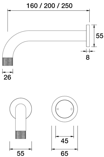
IDK Wall Bath Mixer Set. 200mm outlet A38.043.2.40 - Rumbled Brass
