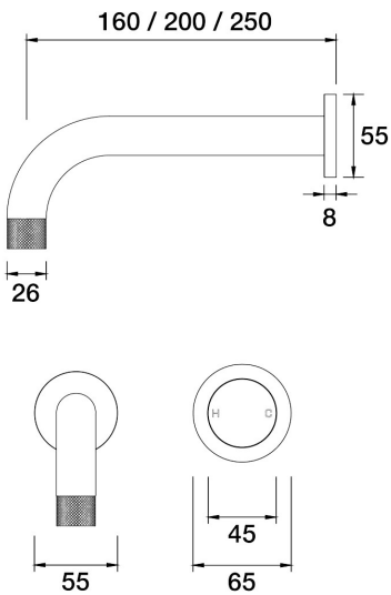
IDK Wall Bath Mixer Set. 200mm outlet A38.043.2.43 - Brass
