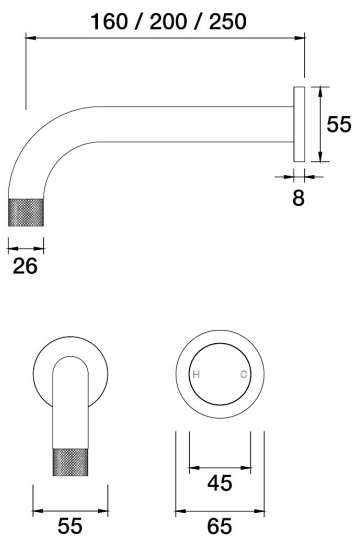
IDK Wall Bath Mixer Set. 250mm outlet A38.043.3.25 - Brushed Nickel
