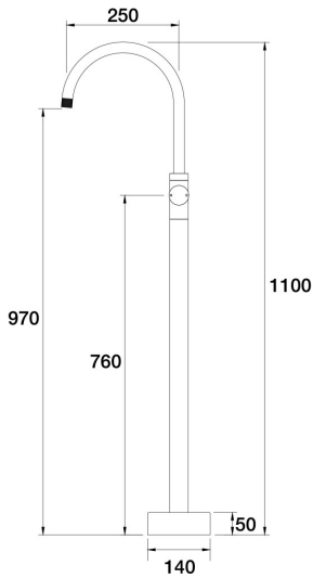
IDK Floor Bath Filler Mixer - Gooseneck A38.072.1.27 - Satin Pearl
