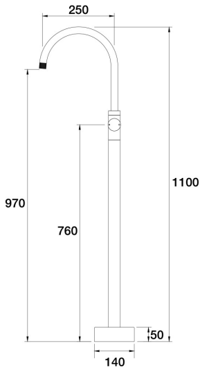
IDK Floor Bath Filler Mixer - Gooseneck A38.072.1.34 - Matt Black
