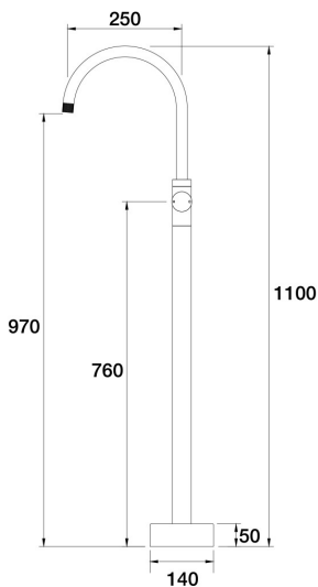
IDK Floor Bath Filler Mixer - Gooseneck A38.072.1.52 - Burnished
