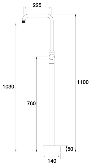
IDK Floor Bath Filler Mixer - 90 Degree A38.073.1.40 - Rumbled Brass
