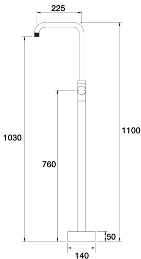
IDK Floor Bath Filler Mixer - 90 Degree A38.073.1.48 - Copper
