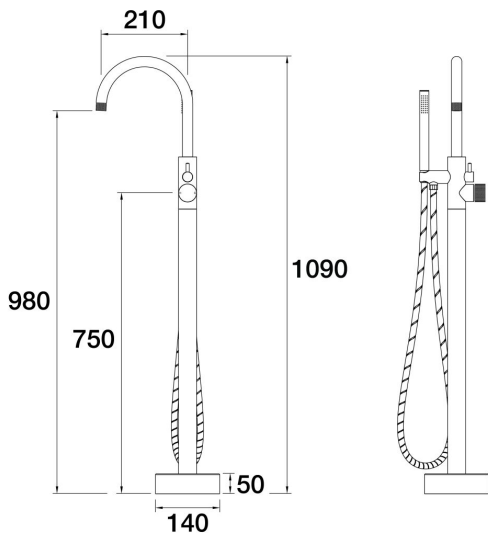
IDK Floor Bath Filler Mixer with Handshower Gooseneck A38.075.1.01 - Chrome
