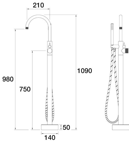
IDK Floor Bath Filler Mixer with Handshower Gooseneck A38.075.1.75 - Forest Mist
