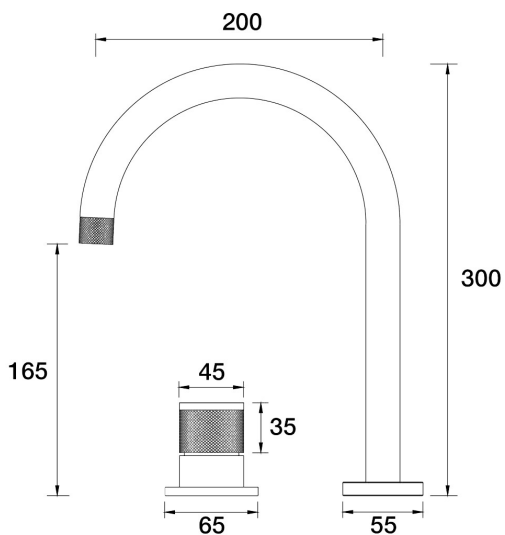
IDK Hob Mixer Set A38.081.2.43 - Brass
