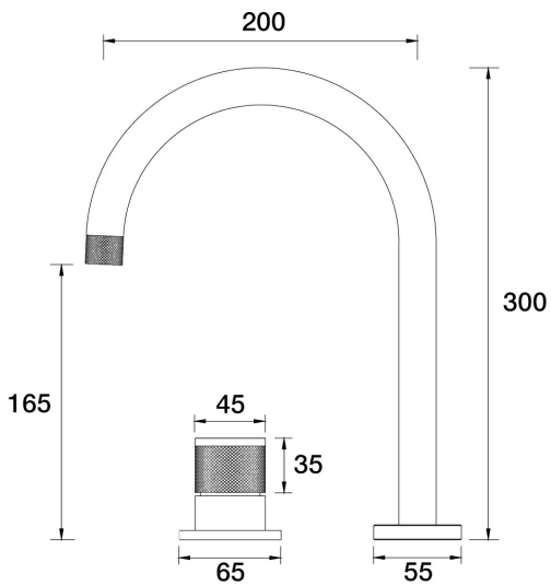
IDK Hob Mixer Set A38.081.2.54 - Volcanic Grey
