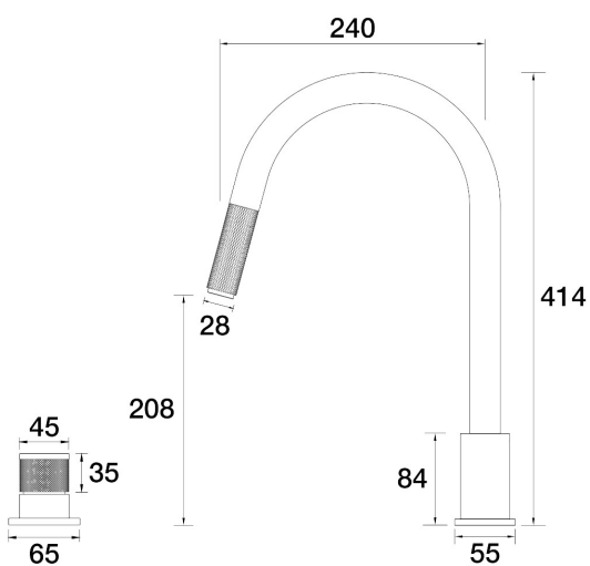
IDK Hob Mixer Pullout Gooseneck Set A38.081.3.19 - 23k Brushed Brass Gold
