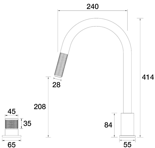
IDK Hob Mixer Pullout Gooseneck Set A38.081.3.67 - Vintage Brass
