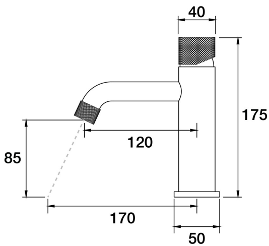
IDK Marble Hob Basin Mixer Carrara Marble A39.011.1.75 - Forest Mist
