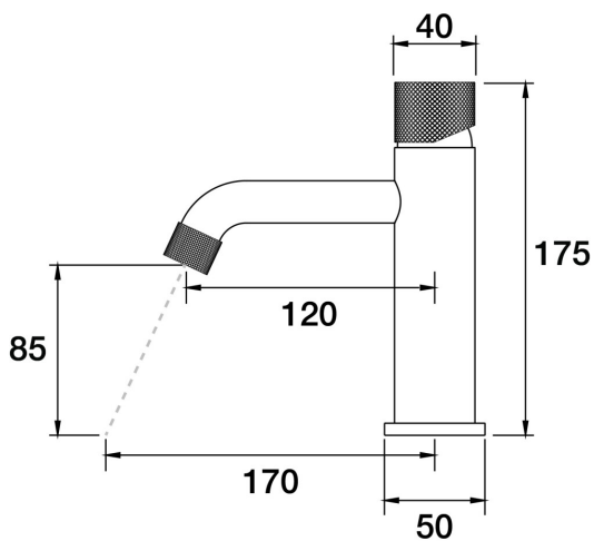
IDK Marble Hob Basin Mixer Nero Marquina Marble A39.011.2.45 - Native Brass
