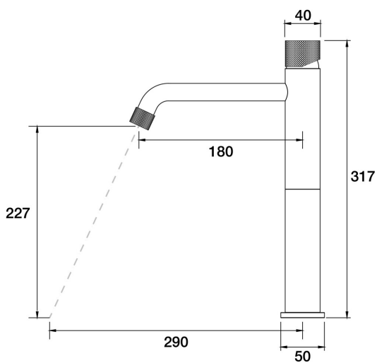
IDK Marble Hob Basin Tower Mixer Nero Marquina Marble A39.012.2.23 - Gunmetal
