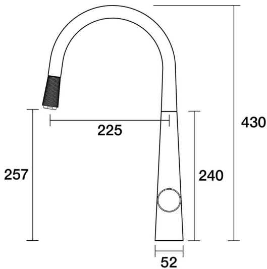
IDK Marble Sink Pull-Out Mixer Carrara Marble A39.024.1.21 - Brushed Rose Gold
