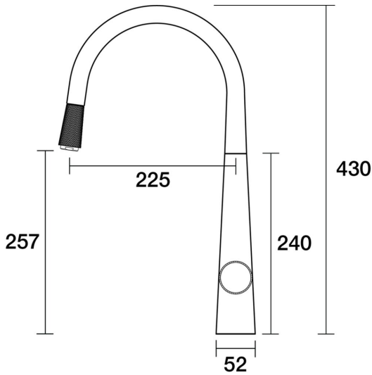
IDK Marble Sink Pull-Out Mixer Nero Marble A39.024.2.01 - Chrome
