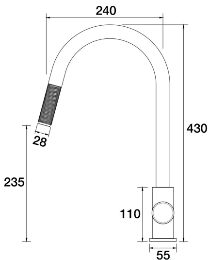
IDK Marble Sink Pull-Out Mixer Gooseneck Nero Marquina Marble A39.024.4.26 - Black Sapphire
