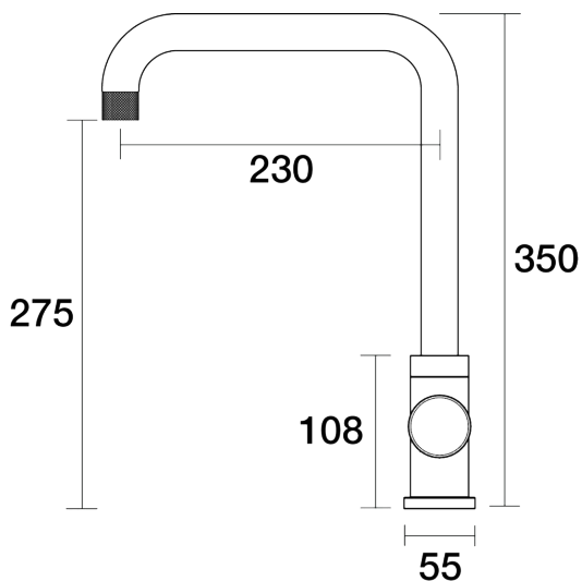
IDK Marble Sink 90 Degree Mixer Bianco Marble A39.025.1.01 - Chrome
