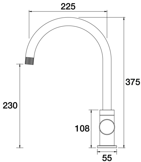
IDK Marble Sink Gooseneck Mixer Nero Marquina Marble A39.026.2.32 - Midnight Black
