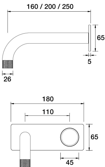
IDK Marble Wall Mixer Basin Set Carrara Marble 160mm outlet Incl. plate A39.032.2.70 - Sea Spray
