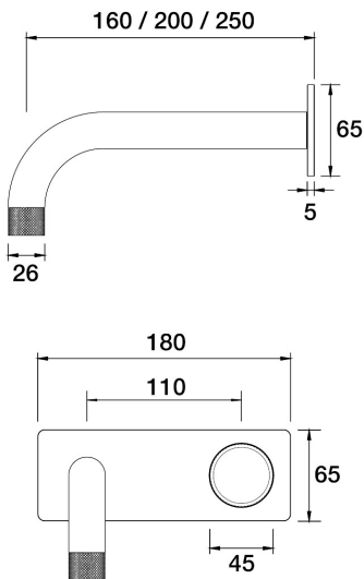
IDK Marble Wall Mixer Basin Set Nero Marquina Marble 200mm outlet Incl. plate A39.032.4.67 - Vintage Brass
