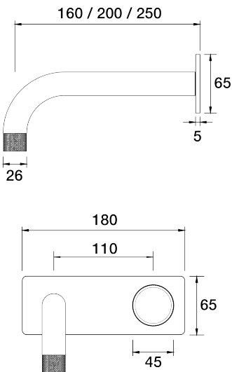
IDK Marble Wall Mixer Basin Set Nero Marble 160mm outlet Incl. plate A39.032.5.01 - Chrome
