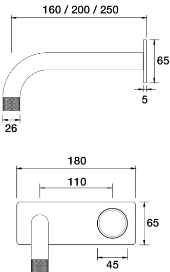
IDK Marble Wall Mixer Basin Set Nero Marquina Marble 160mm outlet Incl. plate A39.032.5.43 - Brass
