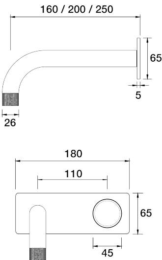
IDK Marble Wall Mixer Basin Set Nero Marble 250mm outlet Incl. plate A39.032.6.01 - Chrome
