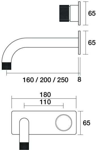
IDK Marble Wall Mixer Basin Set Nero Marble 250mm outlet Incl. plate A39.032.6.01 - Chrome
