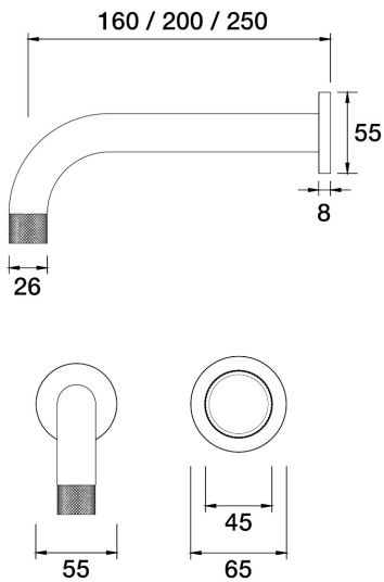
IDK Marble Wall Mixer Basin Set Carrara Marble 160mm outlet A39.033.2.39 - Antique Bronze
