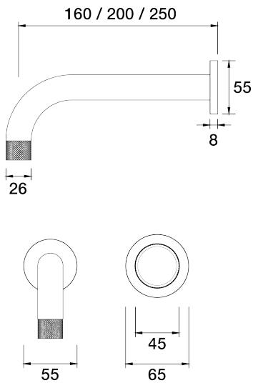
IDK Marble Wall Mixer Basin Set Nero Marble 160mm outlet A39.033.5.01 - Chrome
