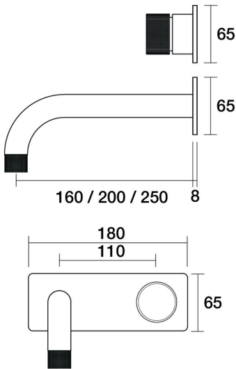
IDK Marble Wall Bath Mixer Set Nero Marble 160mm outlet Incl. plate A39.041.4.01 - Chrome
