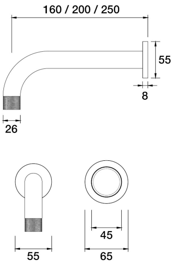
IDK Marble Wall Bath Mixer Basin Set. Carrara Marble 160mm outlet A39.043.1.40 - Rumbled Brass
