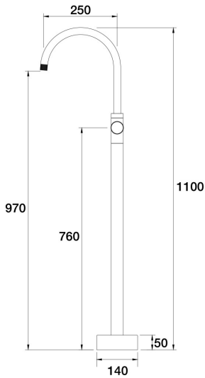
IDK Marble Floor Bath Filler Mixer - Gooseneck Nero Marquina Marble A39.072.2.23 - Gunmetal
