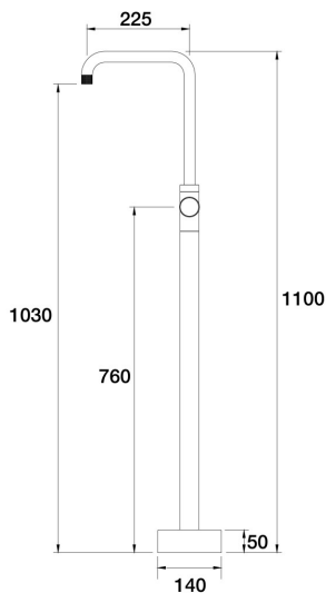
IDK Marble Floor Bath Filler Mixer - 90 Degree Nero Marquina Marble A39.073.2.01 - Chrome
