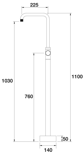
IDK Marble Floor Bath Filler Mixer - 90 Degree Nero Marquina Marble A39.073.2.27 - Satin Pearl
