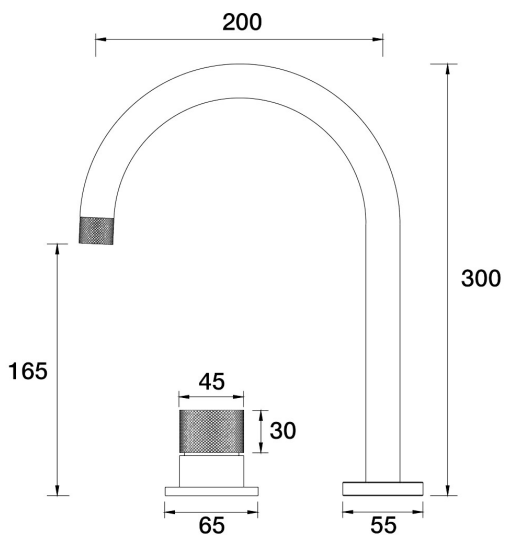
IDK Marble Hob Mixer Carrara Marble Set A39.081.3.43 - Brass
