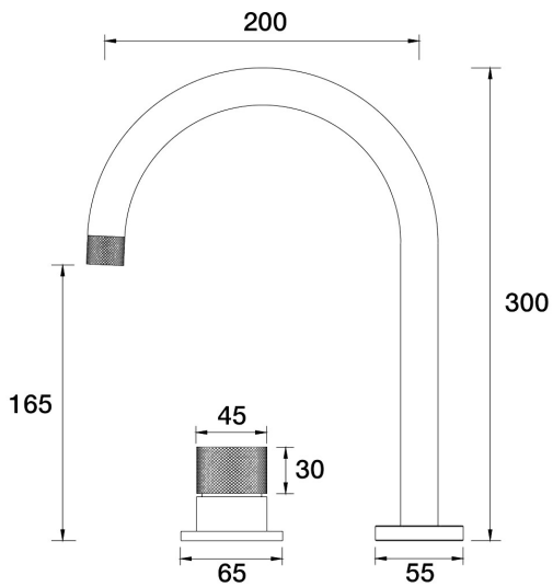
IDK Marble Hob Mixer Nero Marquina Marble Set A39.081.4.39 - Antique Bronze
