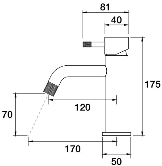
Elm Hob Basin Mixer A40.011.2.43 - Brass
