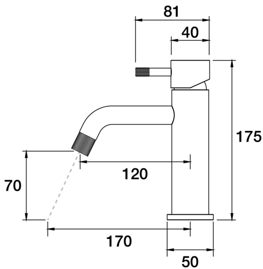
Elm Hob Basin Mixer A40.011.2.57 - Matt Nickel
