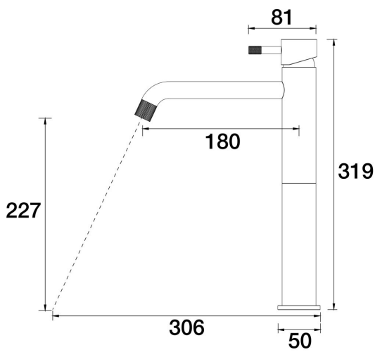
Elm Hob Basin Tower Mixer A40.012.1.01 - Chrome
