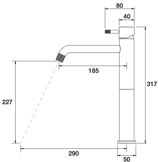
Elm Hob Basin Tower Mixer A40.012.1.27 - Satin Pearl
