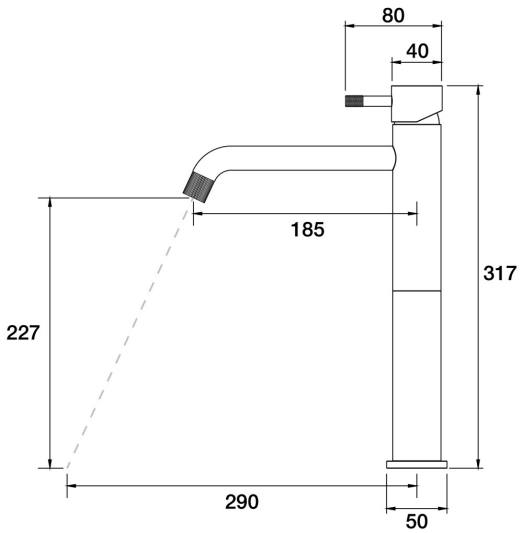
Elm Hob Basin Tower Mixer A40.012.1.41 - Brushed Brass
