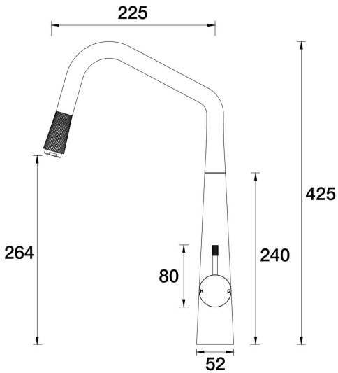
Elm Sink Pull-Out Mixer A40.024.1.01 - Chrome
