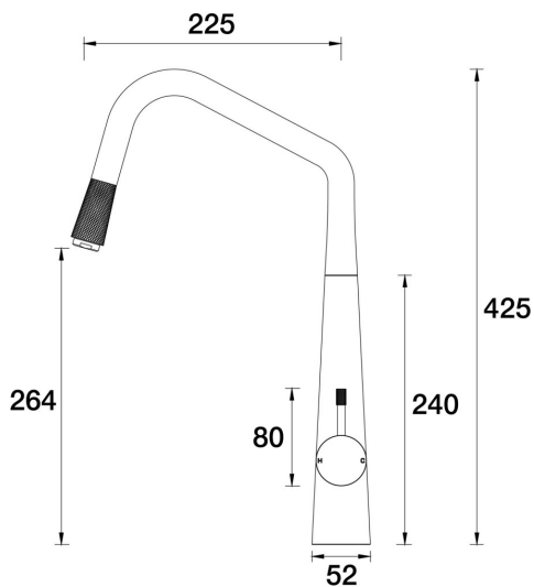
Elm Sink Pull-Out Mixer A40.024.1.34 - Matt Black
