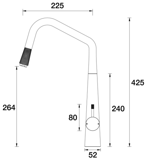
Elm Sink Pull-Out Mixer A40.024.1.44 - Antique Copper
