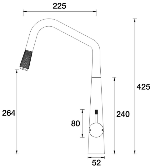
Elm Sink Pull-Out Mixer A40.024.1.57 - Matt Nickel
