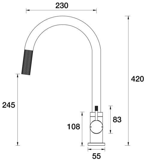
Elm Sink Pull-Out Mixer Gooseneck A40.024.2.01 - Chrome
